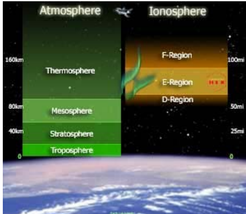
The Earth's atmosphere and ionosphere
